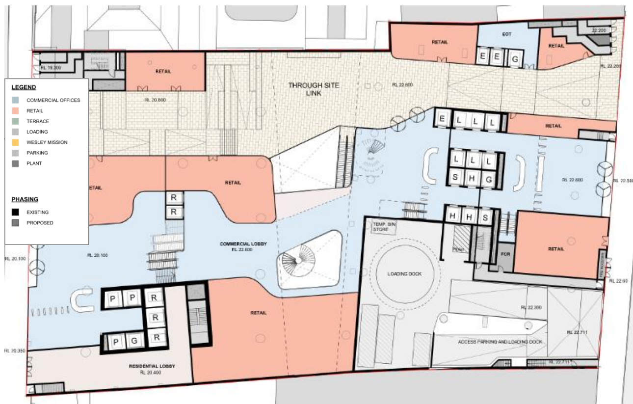
Figure 2: Stockland Piccadilly Complex – Concept Reference Design - Ground plan
